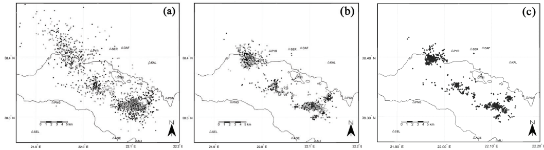
Fig. 5 (a): automatically located epicenters of multiplet clusters belonging to groups D, E and F (year 2006); (b): the same events relocated using the Master Events method; (c): final relocation with a double-difference technique (HypoDD).
