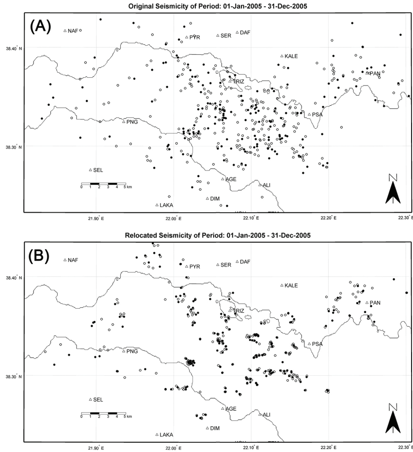
Fig. 4 (A): automatically located epicenters of multiplet clusters belonging to group C (year 2005); (B): the same events relocated using the Master Events method and HypoDD. Master Events are represented by filled circles while slave events are represented by hollow ones.
