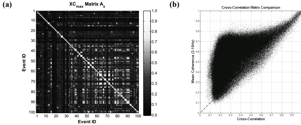
Fig. 2: (a) Cross-correlation matrix for the first 100 events of Group A_s ; (b) element-by-element comparison between cross-correlation ( XC_{max} , horizontal axis) and mean coherence ( m_{coh} , vertical axis) matrices for Group A_s .
