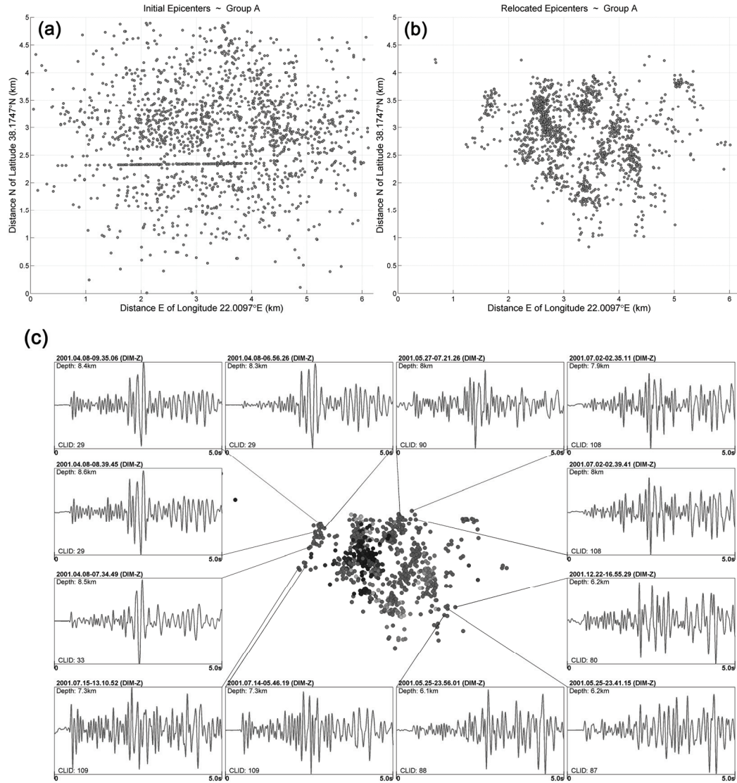
Fig. 6 (a): initial locations of earthquakes in Group A; (b): relocated epicenters using the double-difference method; (c): seismic recordings of the vertical component of station DIM for certain events of Group A. CLID number is the Cluster-ID to which each event belongs. Waveform recordings of events with the same Cluster-ID are similar.
